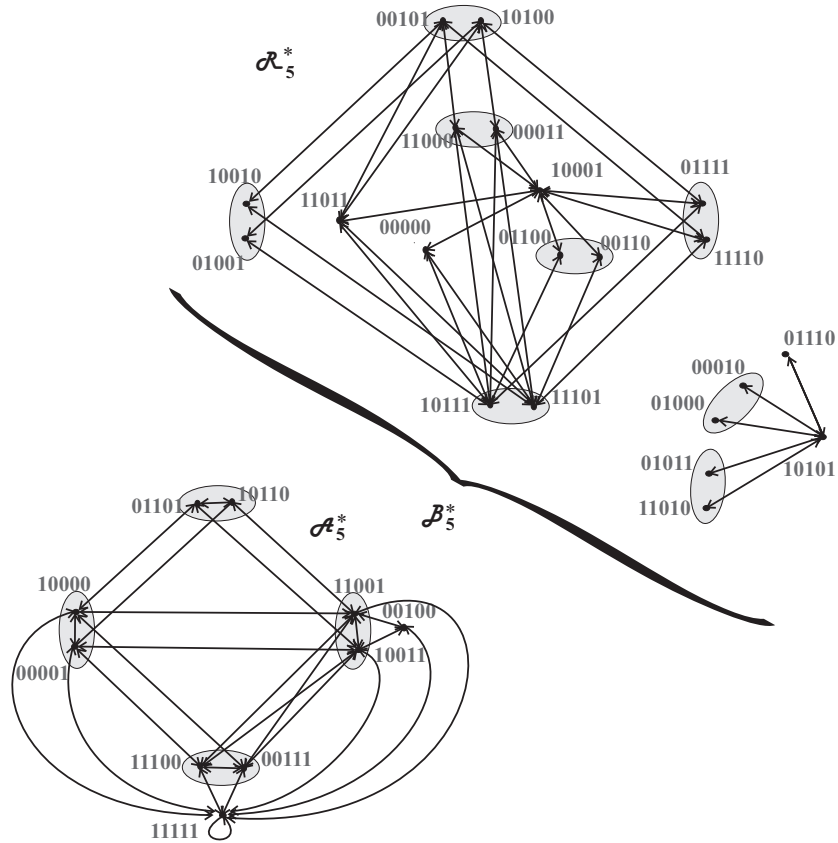
FIGURE 13. Digraph \mathcal{D}_5^*
