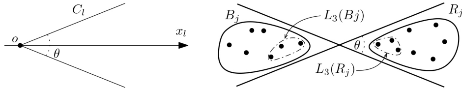
FIGURE 1. The cone C_l and a member (B_j, R_j) of \Psi_l in \mathbb{R}^2 .
