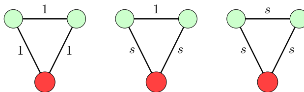
FIGURE 1. Type I, II and III edge labelings
