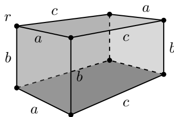
FIGURE 2. The rooted 2-simplicial complex (\mathcal{Q}, r) .
